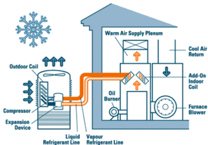
Figure 3: Add-On Heat Pump
