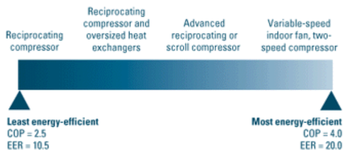
Figure 9: Closed-Loop Earth-energy System Efficiency (at an entering antifreeze water temperature of 0°C)
