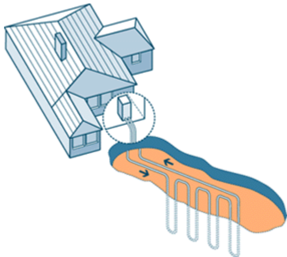
Figure 11: Closed-Loop, Single U-bend Vertical Configuration
