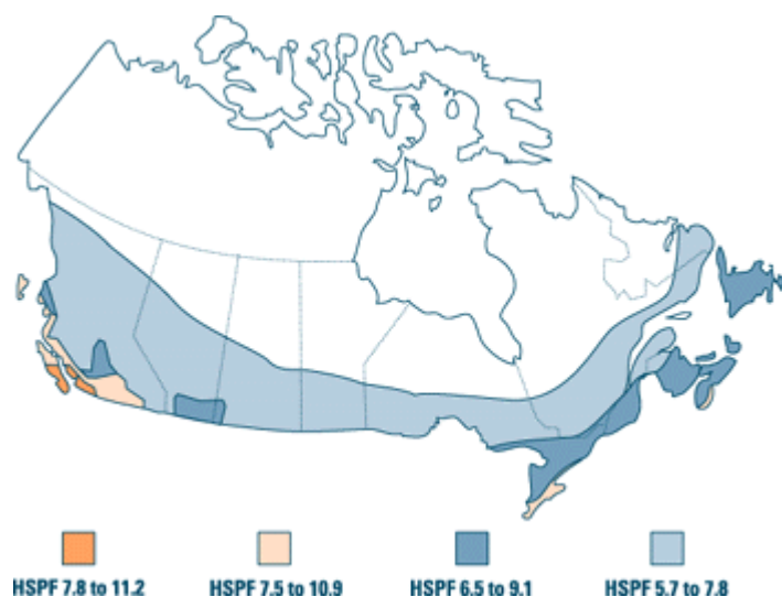
Figure 14: Heating Seasonal Performance Factors (HSPF) for Closed-Loop EESs in Canada.
