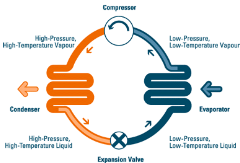
Figure 1: Basic Heat Pump Cycle
