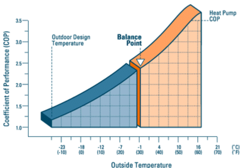
Figure 5: Performance Characteristics of a Typical Air-source Heat Pump
